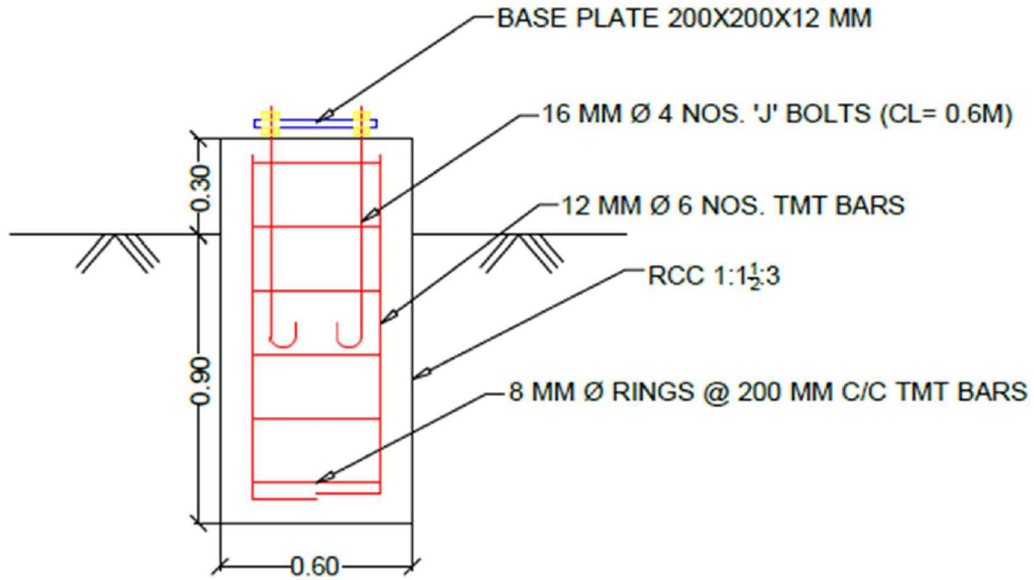
CROSS - SECTION
